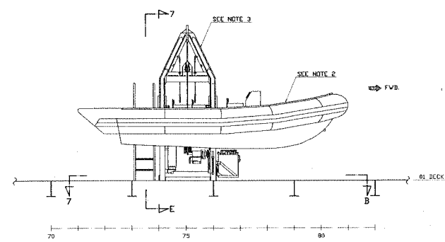
DETAIL 7-C STARBOARD SHOWN 1:50
