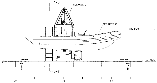
DETAIL 7-C STARBOARD SHOWN 1:50
