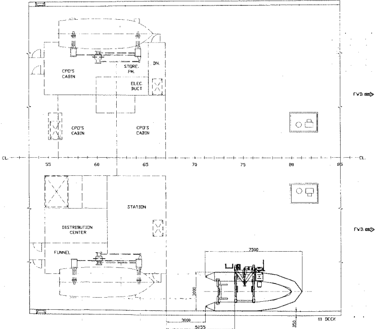
01 DECK PLAN 1:100
