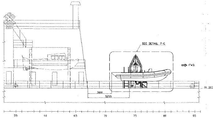
PROFILE 1:100
