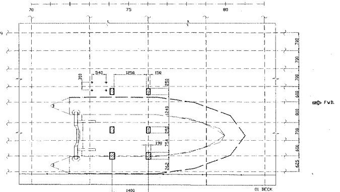
SECTION 7-B STARBOARD SHOWN 1:50
